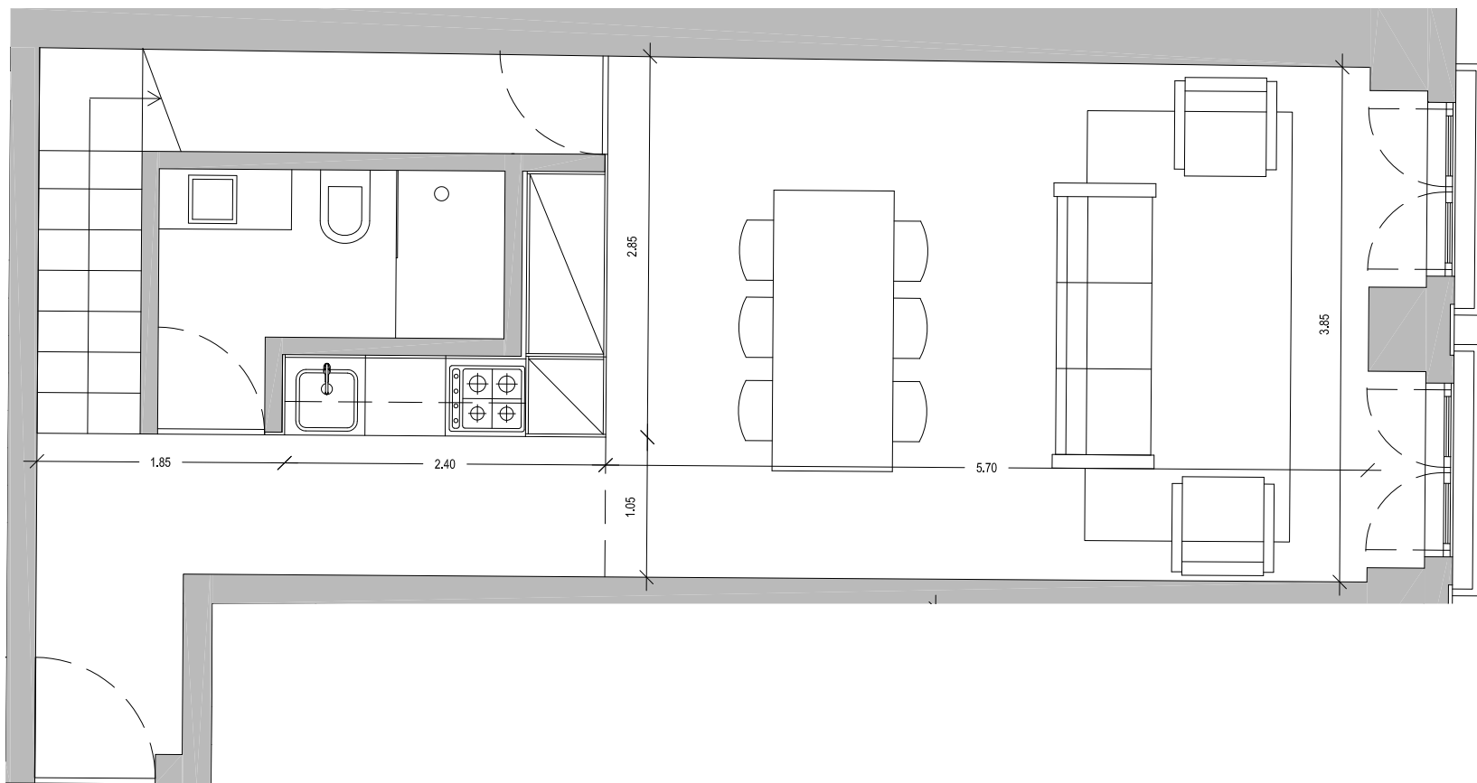
Floor 2A
