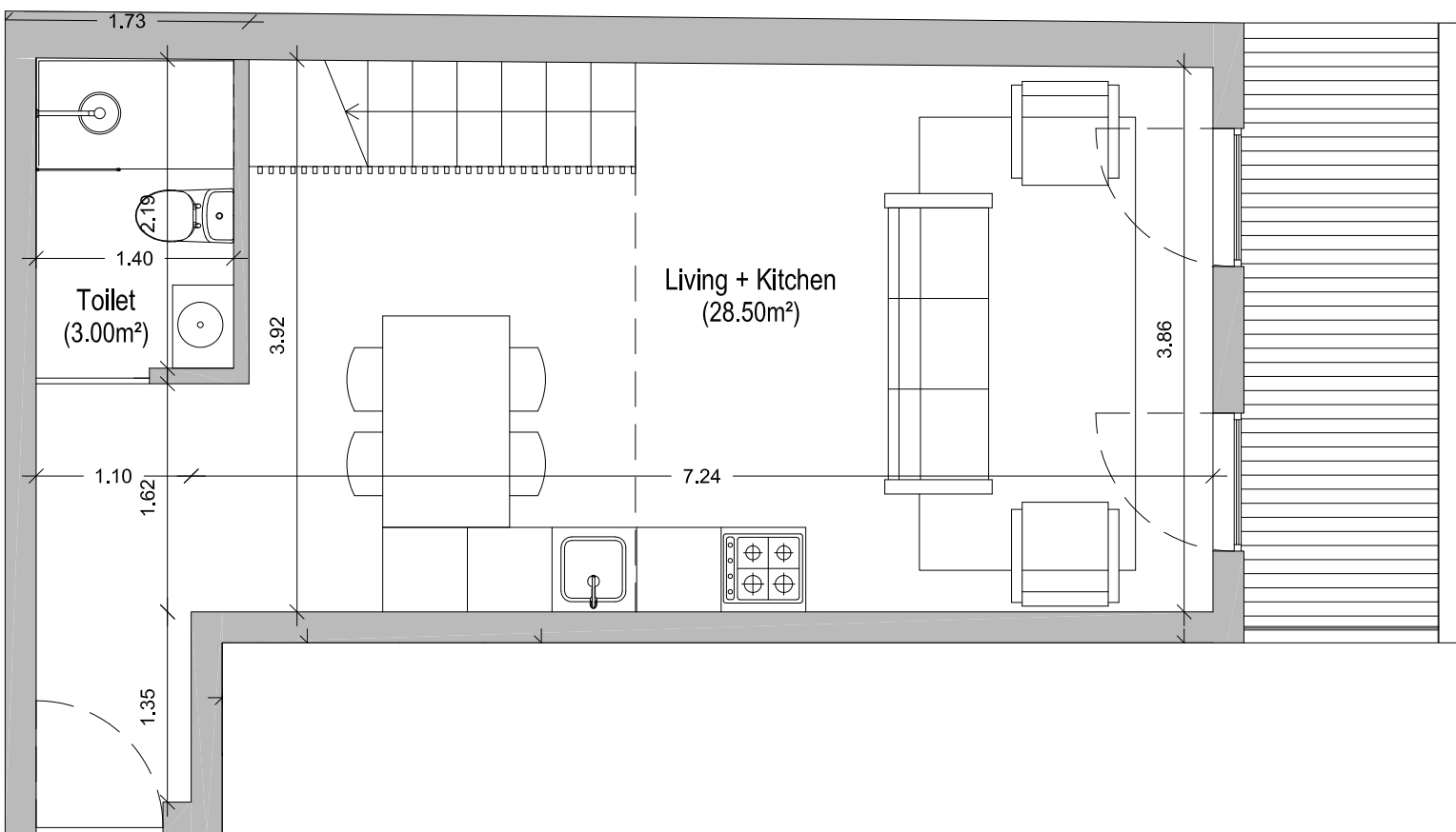
Floor 4A
